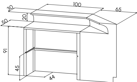
Misure tridimensionali del bancone Counter three-dimensional measures
