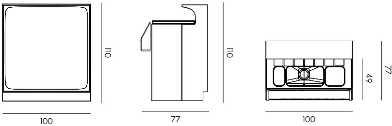
Dublin modulo lineare con cocktail station ABS Dublin straight element with ABS cocktail station
