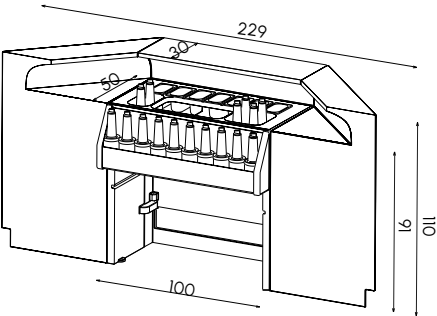
Misure tridimensionali del bancone con cocktail station Counter three-dimensional measures with cocktail station
