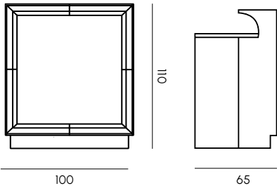
Dublin modulo lineare Dublin straight element
